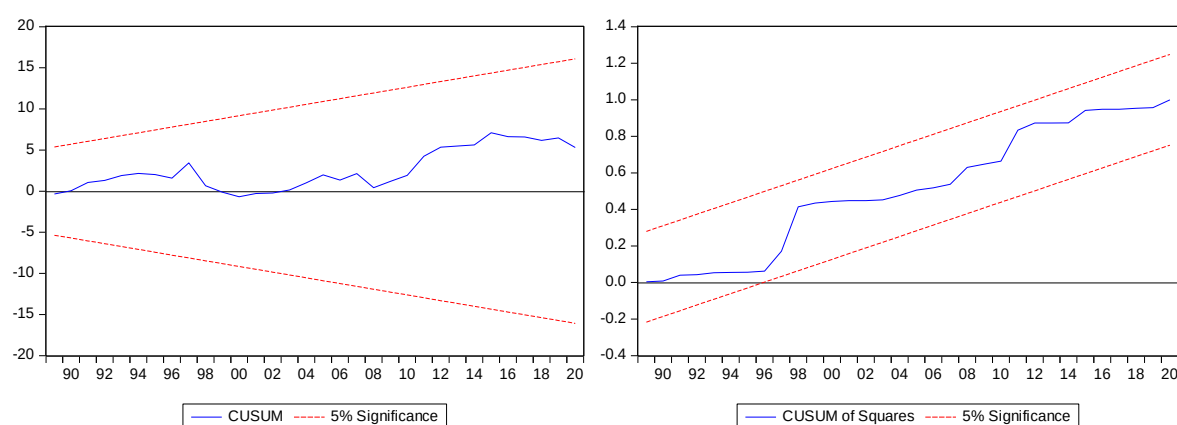
Figure 1. Result of CUSUM and CUSUMSQ test
